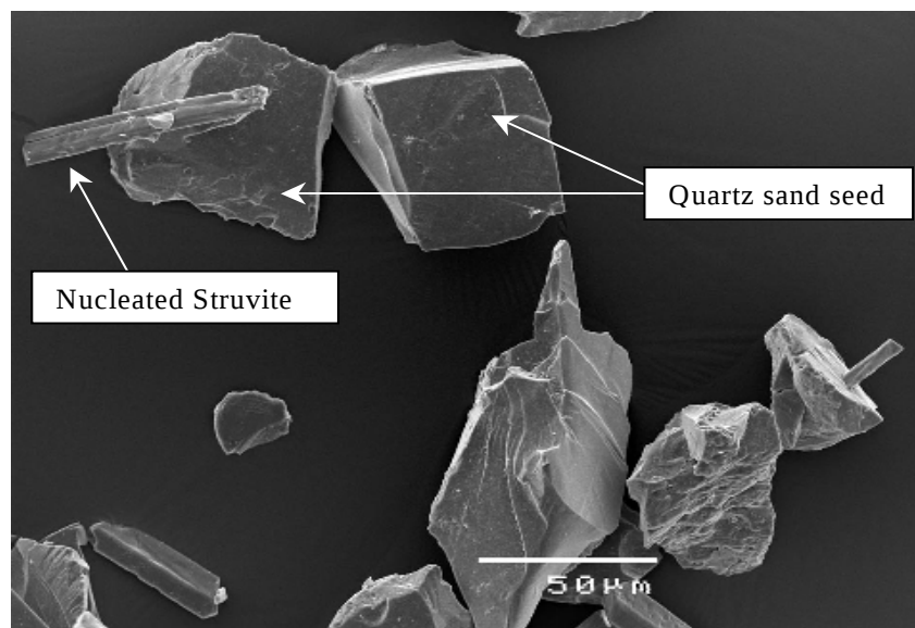
Figure 5.7 Magnified scanning electronic microscopic view of growing struvite and quartz sand seeds
