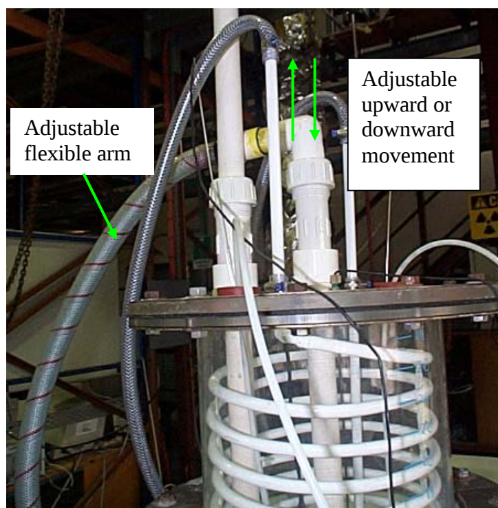
Figure 4. 5 Photographic presentation of adjustable recirculation arm of reactor
