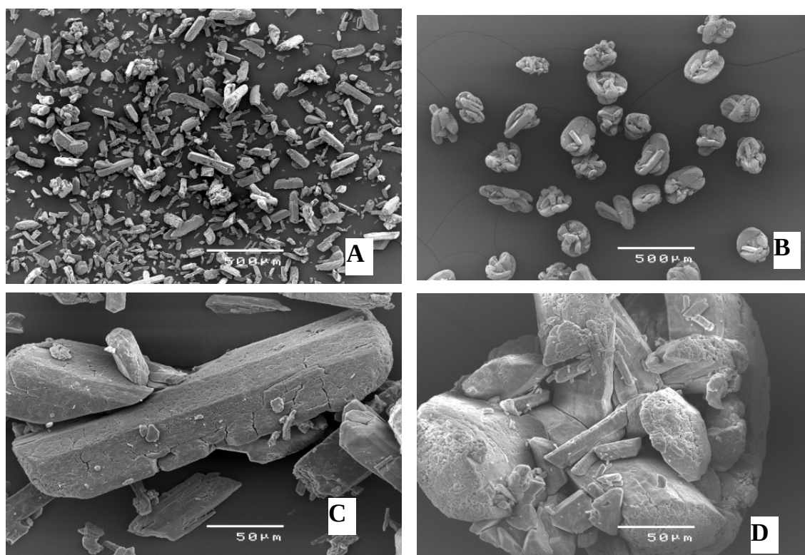
Figure 5. 11 SEM view of air-dried struvite (A); magnified view of air-dry struvite (C); temperature dry (100°C) struvite (B); magnified View of temperature dry struvite (D)
