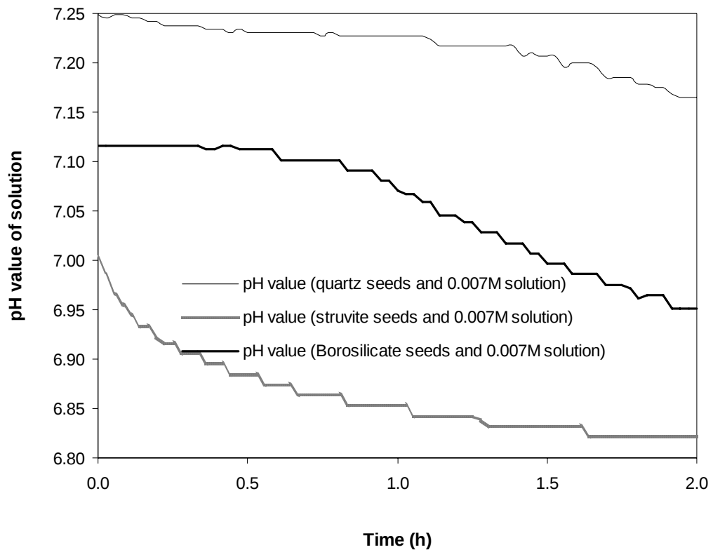
Figure 5. 2 Reaction kinetics during experiment using 0.007 M solution
