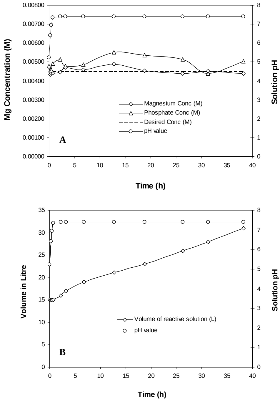
Figure 5. 24 (A) Experimental control; (B) Operating volume in fed-batch action (Expt-2)
