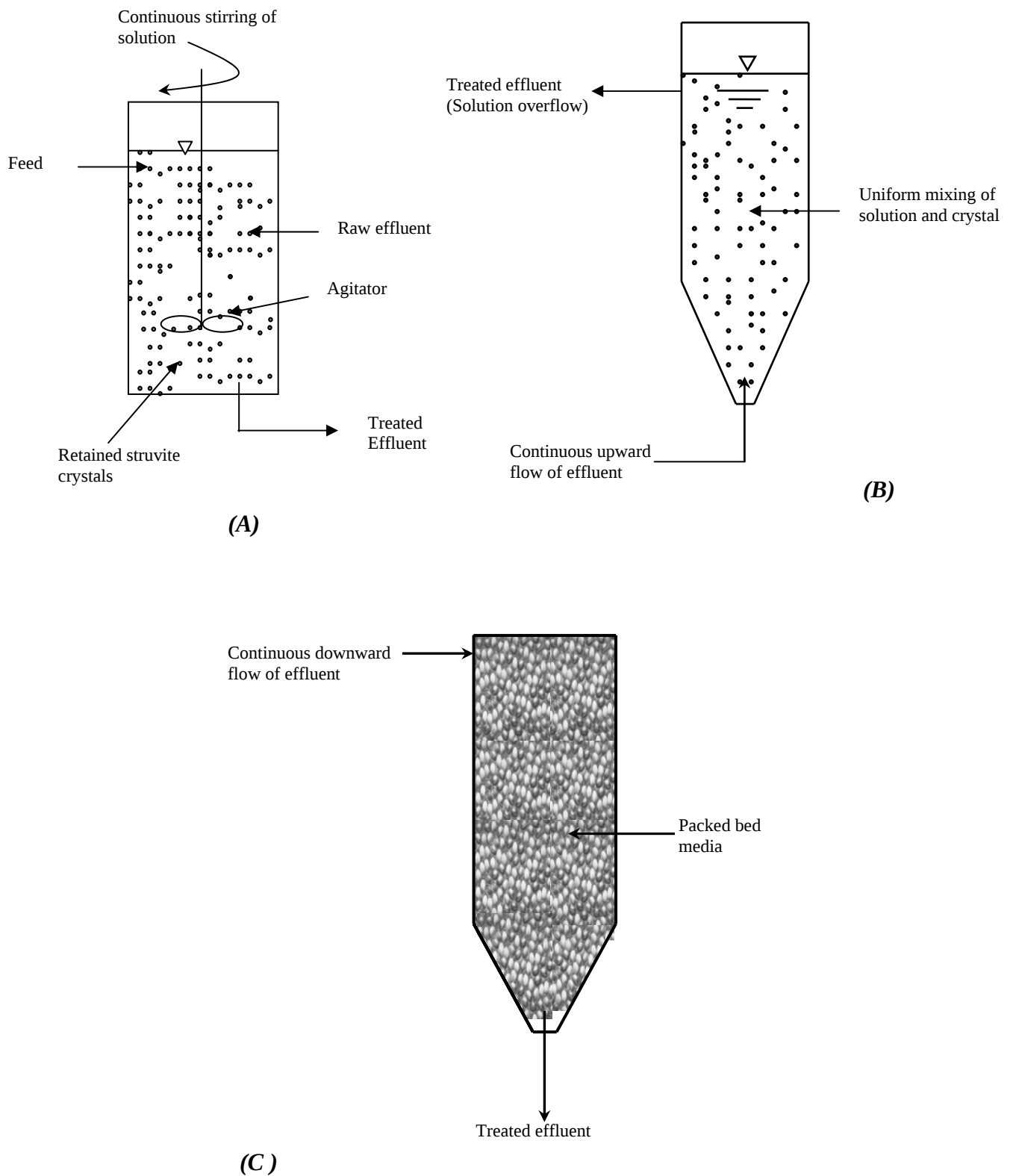
Figure 2. 6 Schematic of MSMPR (A), Fluidized bed reactor (B), and packed bed reactor (C )
