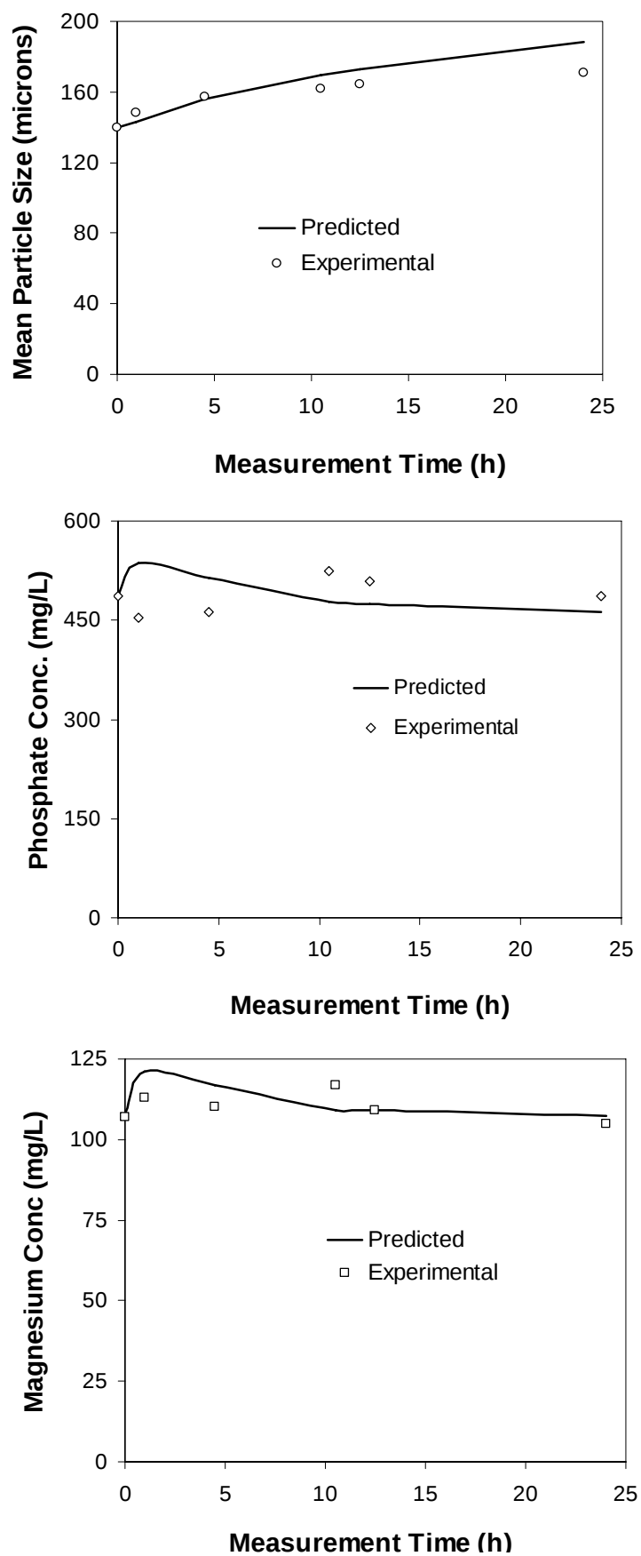
Figure 6. 12 Overlay charts of experiment 1 (Est.type 2)
