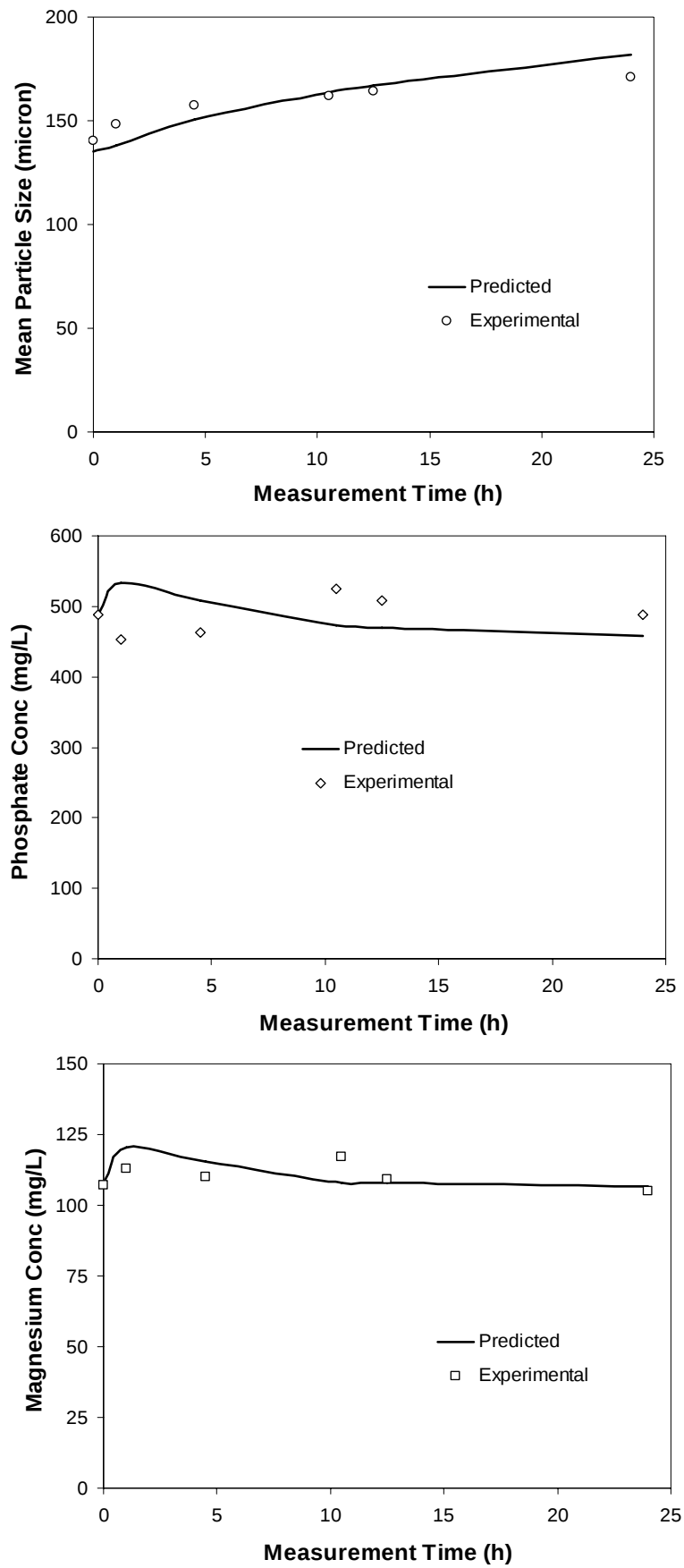
Figure 6. 15 Overlay charts of experiment 1 (Est.type 3)
