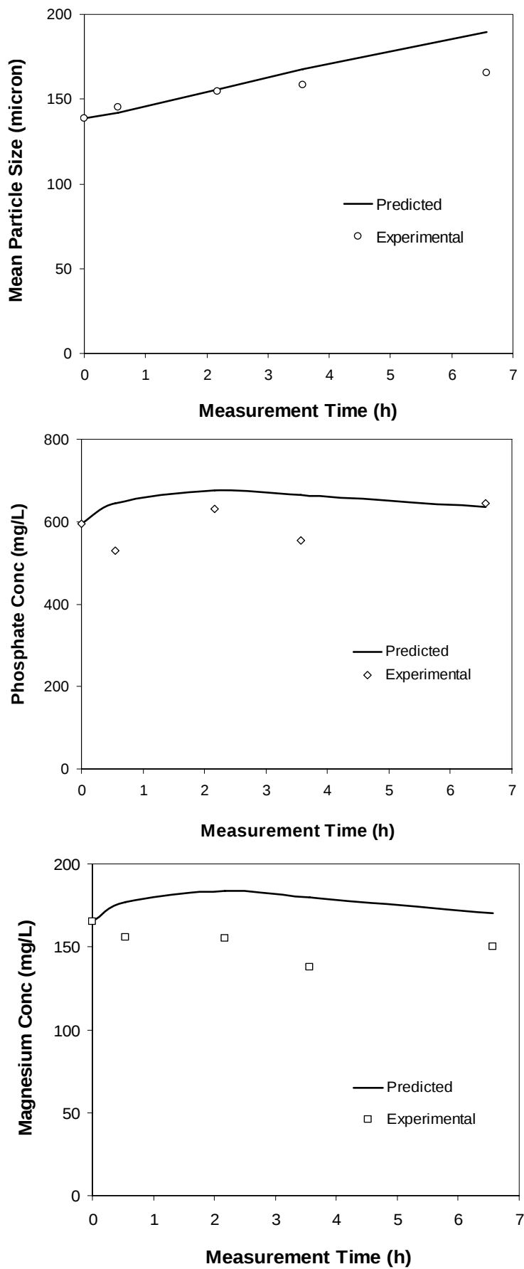
Figure 6. 9 Overlay charts of experiment 2 (Est.type 1)
