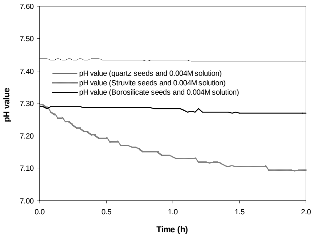
Figure 5. 3 Reaction kinetics during experiment using 0.004 M solution
