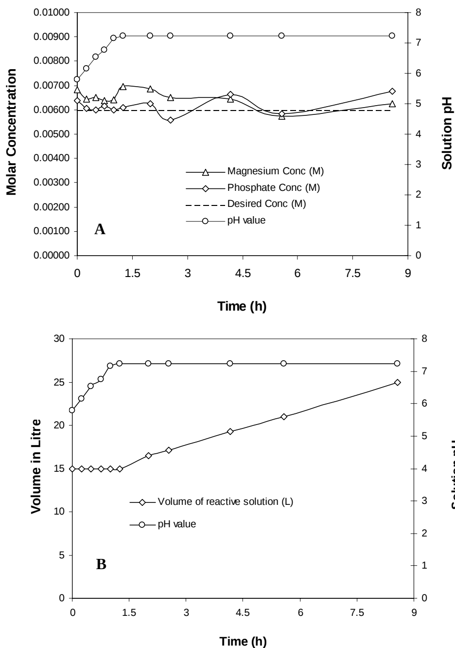
Figure 5. 25 (A) Experimental control; (B) Operating volume in fed-batch action (Expt-3)
