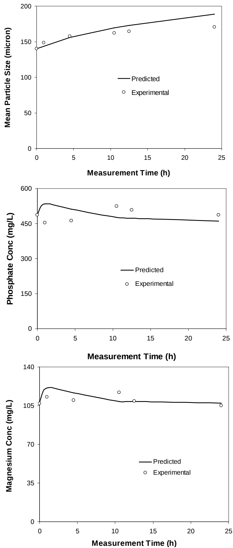
Figure 6.8 Overlay charts of experiment 1 (Est.type 1)
