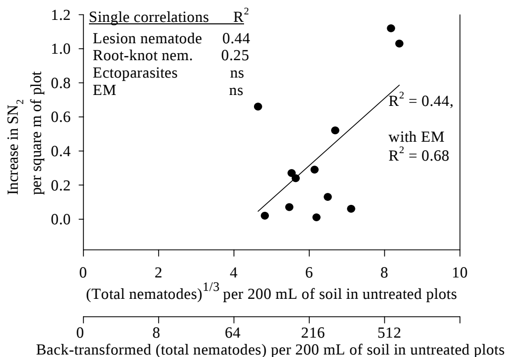
Figure 10.3.7.1: Plant crop increases in established stalks ( SN_2 ) at 200 DAP due to the nematicide, relating to the density of total nematodes (endoparasites + ectoparasites) at planting ( P_i ), and EM.
