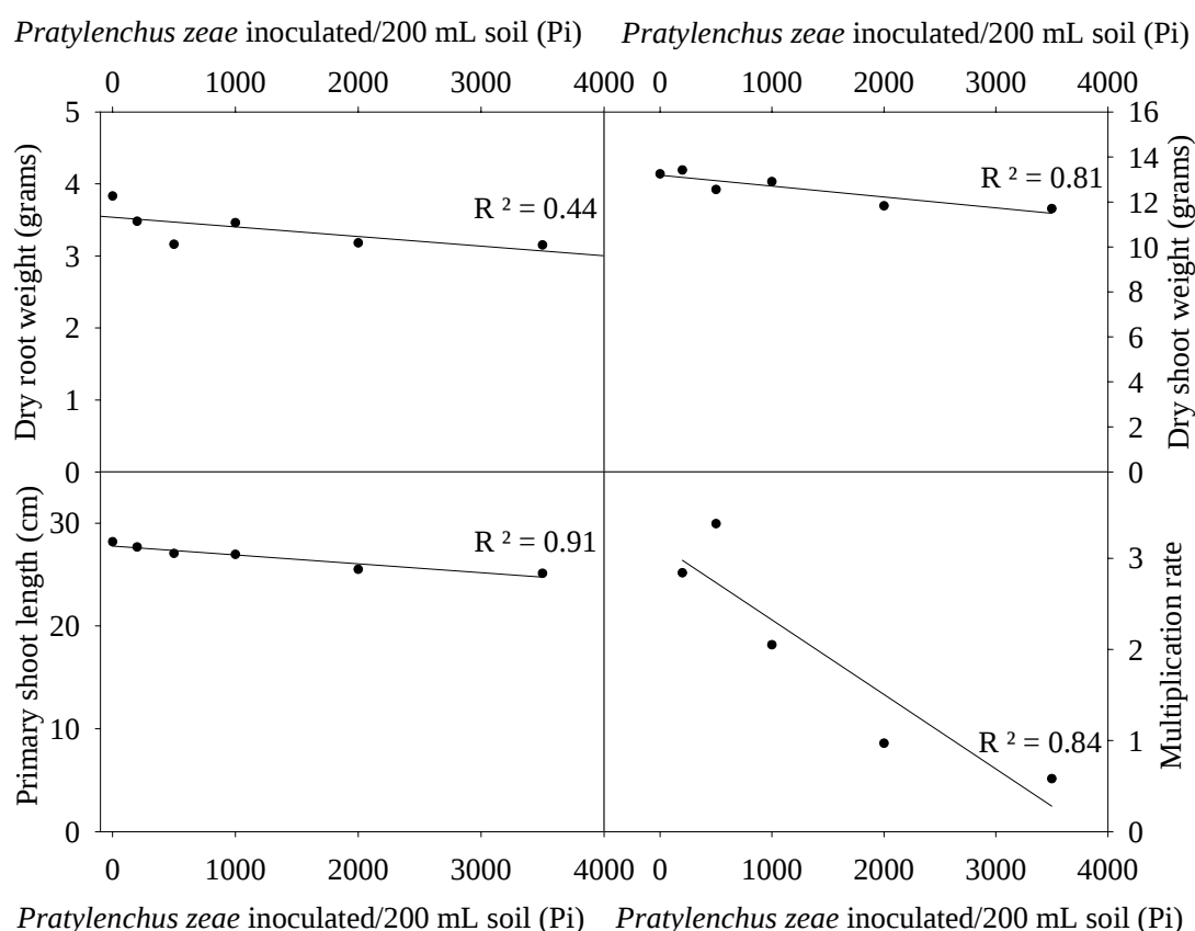
Figure 7.3.3.2: Relationship between the mean inoculum density ( P_i ) of Pratylenchus zeae , mean root and shoot growth, and nematode multiplication.
