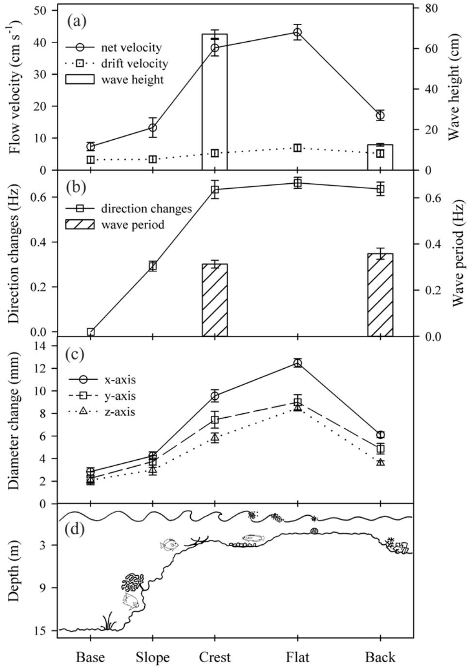
Fig. 1.4. Water motion assessments amongst five habitats on an exposed reef at Lizard Island. (a) Net flow velocities from gypsum dissolution, with drift velocities recorded for each habitat and incident wave heights on the front and back reef for this exposed location. (b) Wave period and rates of flow direction change recorded in each habitat. (c) Diameter change of gypsum balls across three axes. (d) Habitat depths on exposed reef profile. Error bars are standard errors of the mean.
