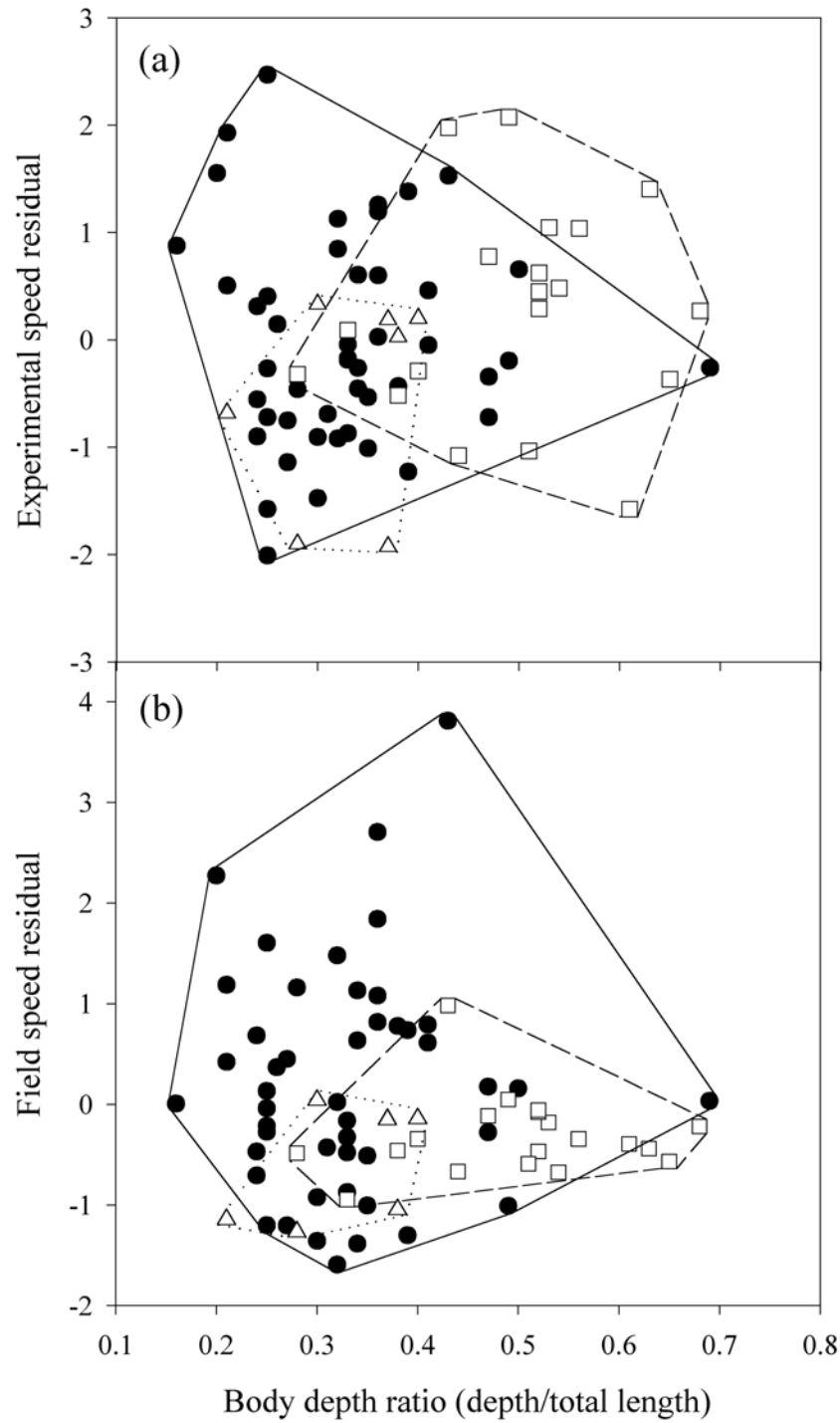
Fig. 2.8. Relationship between body depth and (a) experimental swimming speed, and (b) field swimming speed in 73 species of coral reef fishes. Solid, dashed and dotted lines represent the boundaries for pectoral (circles), pectoral-caudal (squares) and caudal-swimming (triangles) taxa, respectively. Vertical axes have been corrected for body size; high positive values represent high speeds for a given size.
