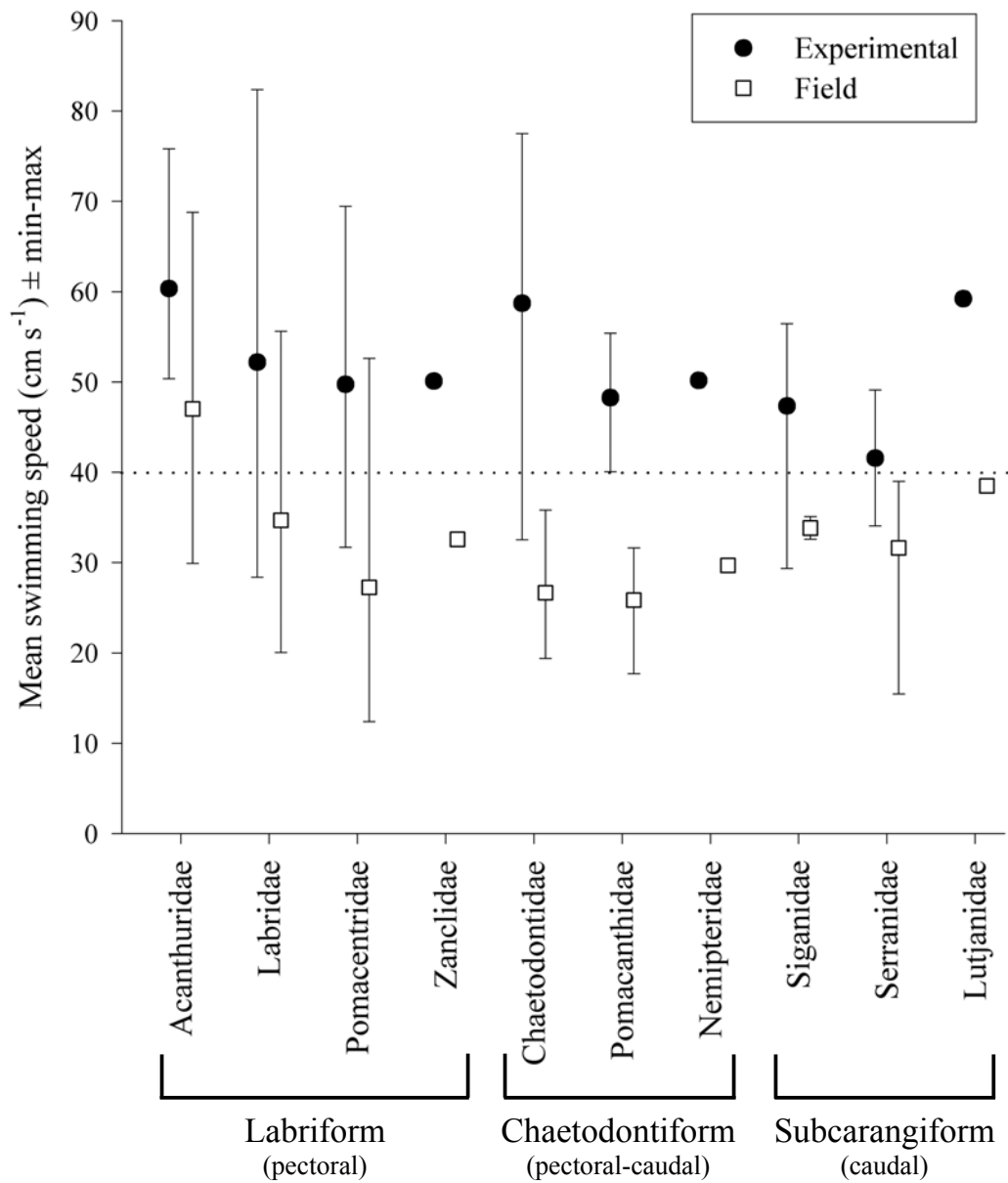
Fig. 2.4. Range of experimental ( U_{crit} ) and field speeds recorded in 10 reef fish families, arranged according to the predominant swimming mode. Each value is the overall mean swimming speed and the minimum and maximum average speed recorded for a species in each family, for both field and experimental performance trials. Note that only those families which have predominantly pectoral-swimming species display absolute field speeds that exceed 40 \text{ cm s}^{-1} (dotted line).
