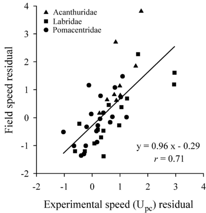
Fig. 4.1. Relationship between field and experimental swimming speed in 44 species of labriform-swimming fishes. Both axes have been corrected for body size; high positive residuals represent high speeds for a given size. Note that the linear regression is close to isometric (slope = 1.0).
