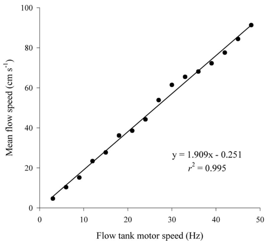
Fig. A2.1. Mean flow speed in working section of the 194 L recirculating flow tank against shaft rotation speed of the 0.75 kW electric motor. Flow speeds are means taken from high speed video tracking of 12 replicate passive particles at each motor speed.
