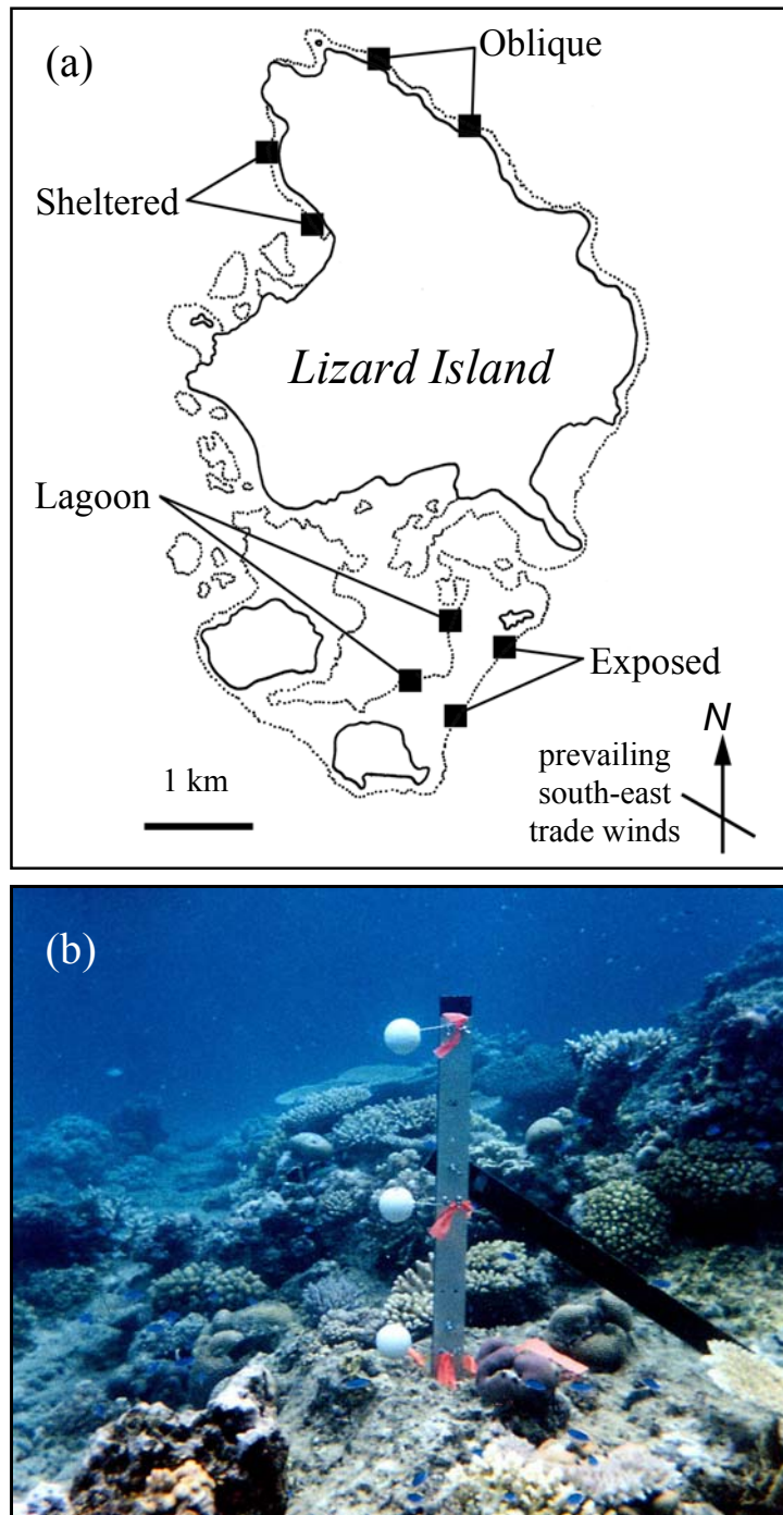
Fig. 1.2. (a) Location of study sites at four wave exposures around Lizard Island ( 14^{\circ}38'S , 145^{\circ}26'E ), Great Barrier Reef, Australia. Depth profile of habitat zones within the exposed locations are presented in Fig. 1.4. (b) Plaster balls deployed on one of the three replicate stakes within the crest habitat of a windward reef site. Data is presented on the topmost plaster ball (60 cm from substratum) to match the average water-column position of reef fishes at these locations (Fulton et al. 2001).
