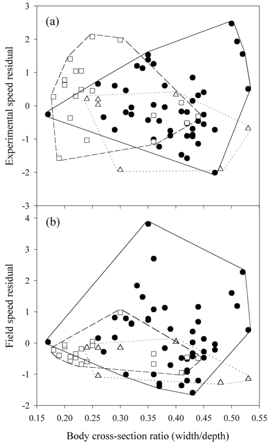
Fig. 2.9. Relationship between body cross-section profile and (a) experimental swimming speed, and (b) field swimming speed in 73 species of coral reef fishes. Solid, dashed and dotted lines represent the boundaries for pectoral (circles), pectoral-caudal (squares) and caudal-swimming (triangles) taxa, respectively. Vertical axes have been corrected for body size; high positive values represent high speeds for a given size.
