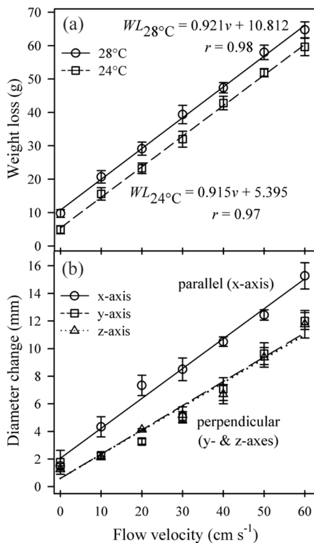
Fig. 1.3. Gypsum dissolution calibration. (a) Weight loss ( WL ) from gypsum balls after 24 hours exposure to seven flow velocities ( v ) at two water temperatures. (b) Diameter change across three axes after 24 hours exposure to seven flow velocities at 24°C. Error bars are standard errors of the mean.
