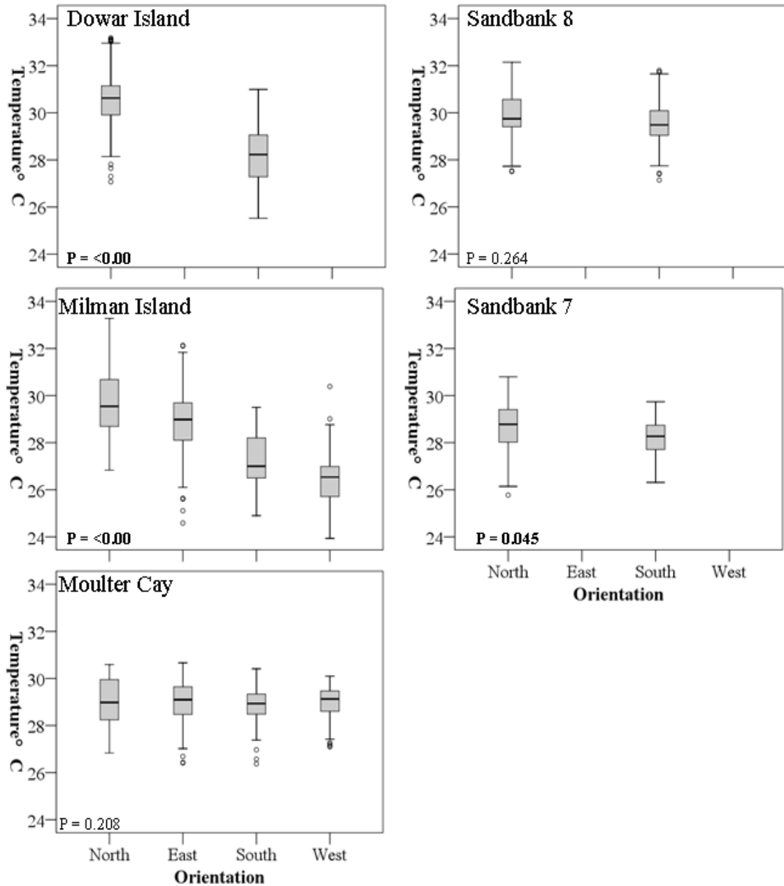
Figure 3.4. Comparison of sand temperature at different beach orientations for the selected nesting grounds used by the northern Great Barrier Reef green turtle population during the 2007-2008 nesting season. Bold indicates a significant difference in sand temperature between the different profiles.
