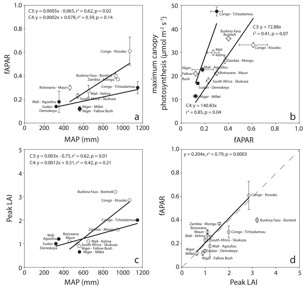
Fig. 9. (a) Relationship of satellite-derived peak f_{\text{APAR}} to mean annual rainfall for all sites in this study \pm SD. The tree dominated ecosystem (white circles, C 3 , n=7 ) differ in slope and intercept from the grasslands (black circles, C 4 , n=4 ) (b) The relationship between maximum canopy photosynthesis ( F_{\text{Pmax}} ) and peak f_{\text{APAR}} for the African sites \pm SD. Sites dominated by C 3 trees have a different (steeper) slope to those dominated by C 4 grasses. (c) A similar dependency as found for peak f_{\text{APAR}} vs. MAP was found for ground measured peak LAI vs. MAP, resulting in slightly different slopes. (d) Correlation between ground based peak LAI and remote sensing based peak f_{\text{APAR}} for 10 African ecosystems \pm SD (the Burkina Faso site was excluded since it seemed to represent an outlier, due to a different technique for estimating LAI). The dashed line represents the 5:1 line.
